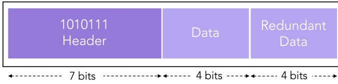
Fig. 5. Data packet structure
