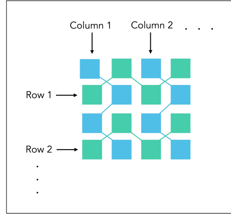
Fig. 3. Touchpad layout
